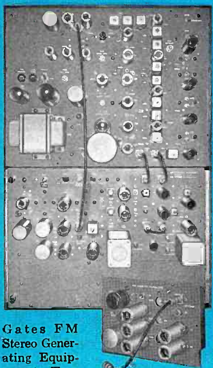
M-6160 Sub-carrier Generator with mute
